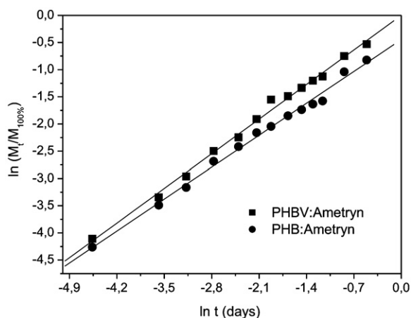
Fig. 5. Results of the analyses of PHB and PHBV microparticles containing ametryn, using the mathematical model of Peppas.
